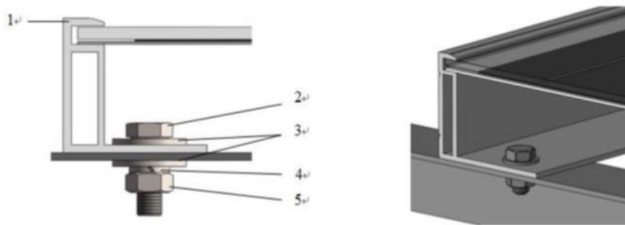
Fig.1 Backsheet-Glass module
