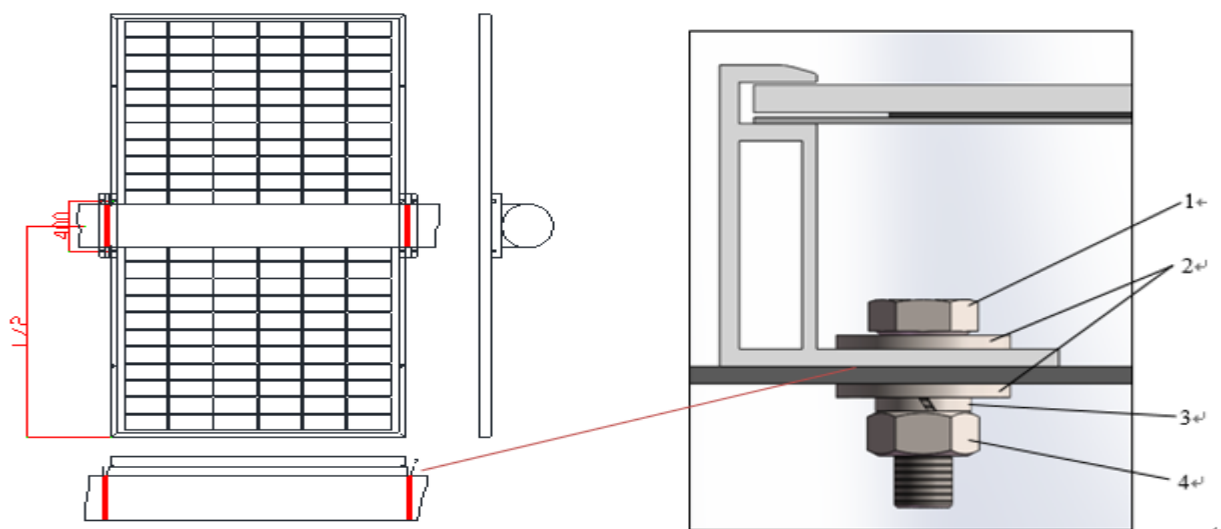
Fig 5. PV module installed with Single-axis Tracing System
