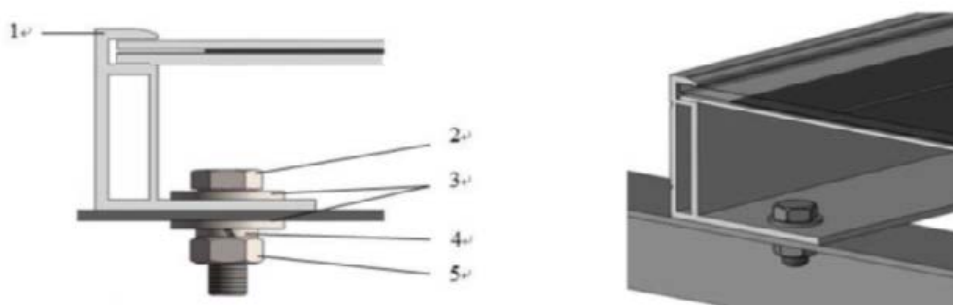
Fig.4 Duomax serial module with frame
