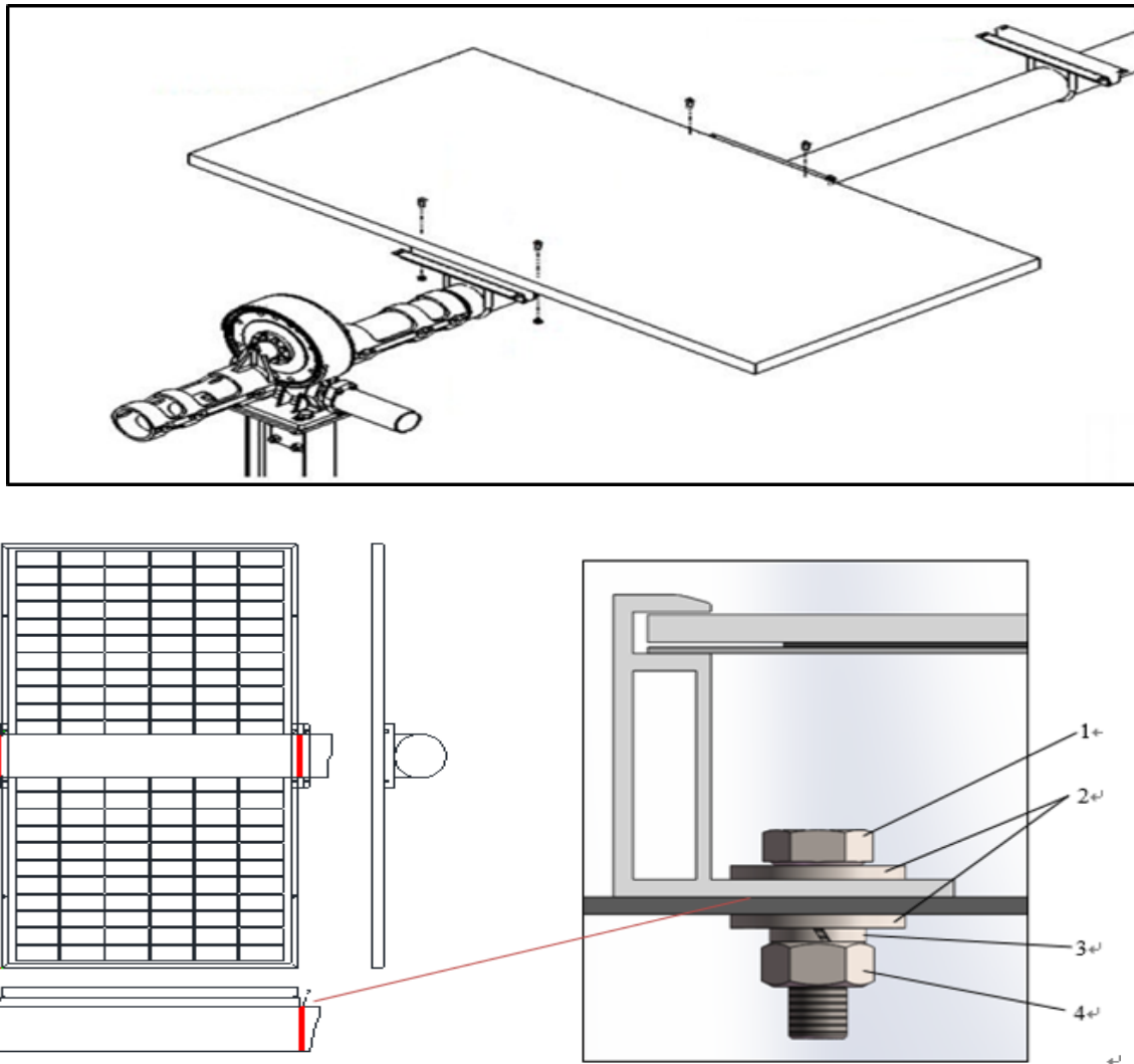
Fig 5. PV module installed with Single-axis Tracing System
