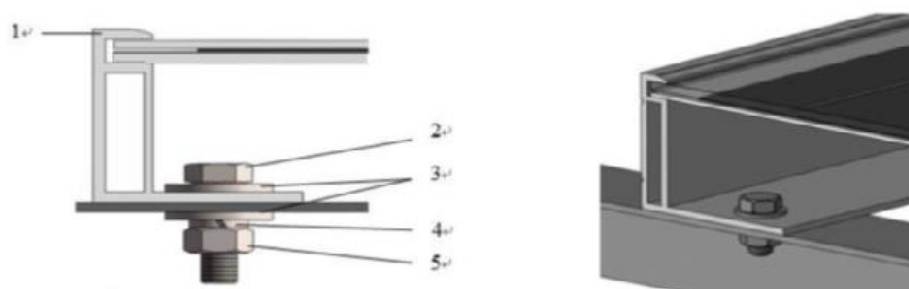
Figure.1 Duomax serial module with frame
