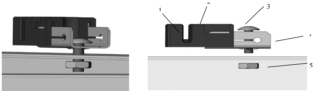
Figure 5. Tyco grounding bolt # 1954381-2 (Not applicable for TRINAMOUNT module series)
