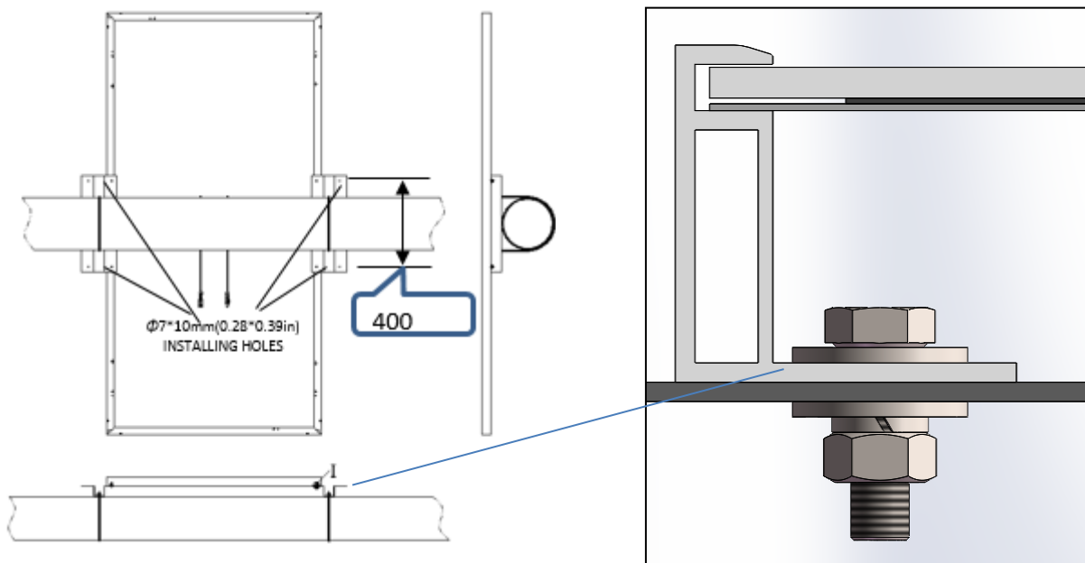
Figure 3. PV module installed with Single-axis Tracing System
