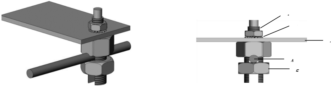
Figure 4. Tyco grounding bolt # 2058729-1
